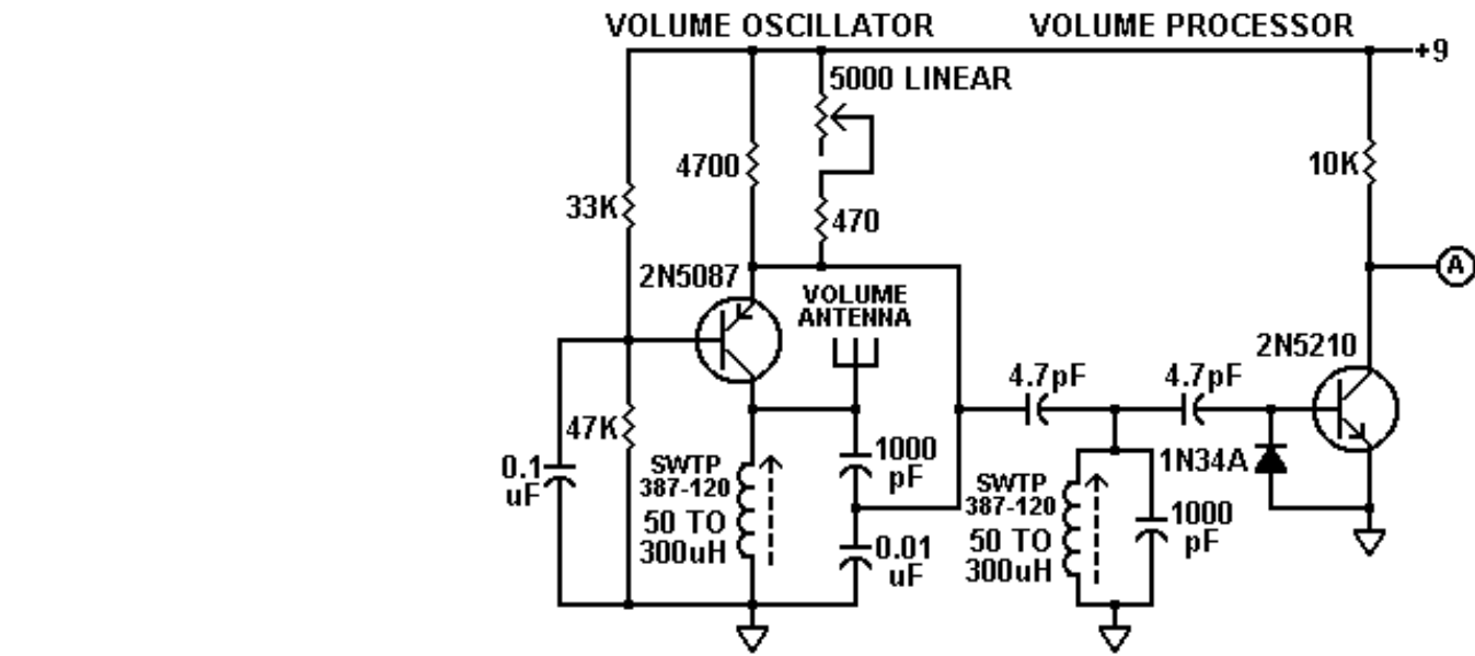
SOUTHWEST TECHNICAL PRODUCTS CORPORATION THEREMIN (KIT NUMBER 142)
