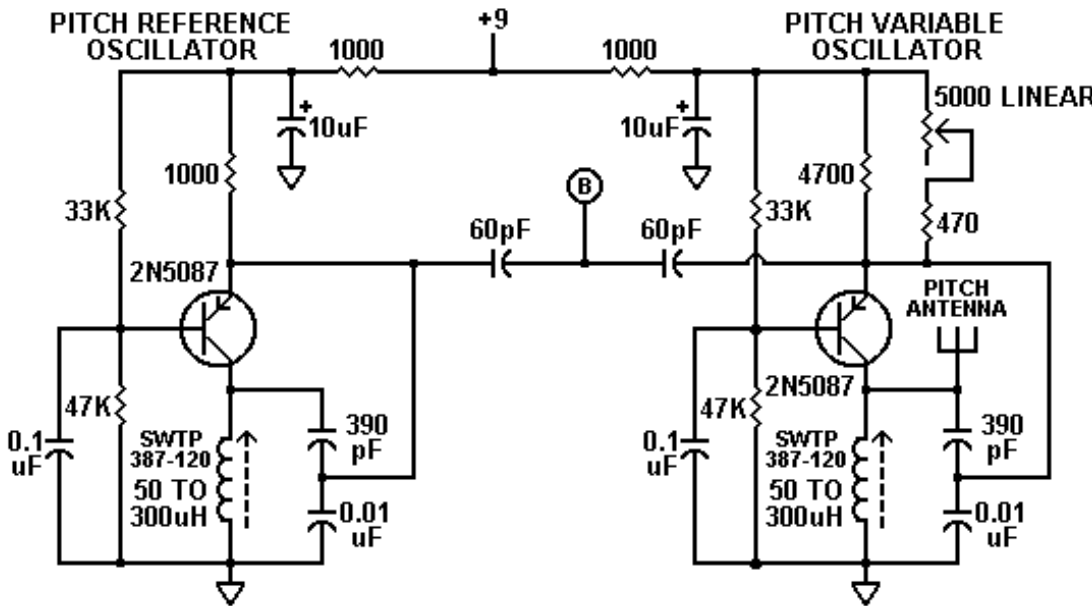
SOUTHWEST TECHNICAL PRODUCTS CORPORATION THEREMIN (KIT NUMBER 142)
