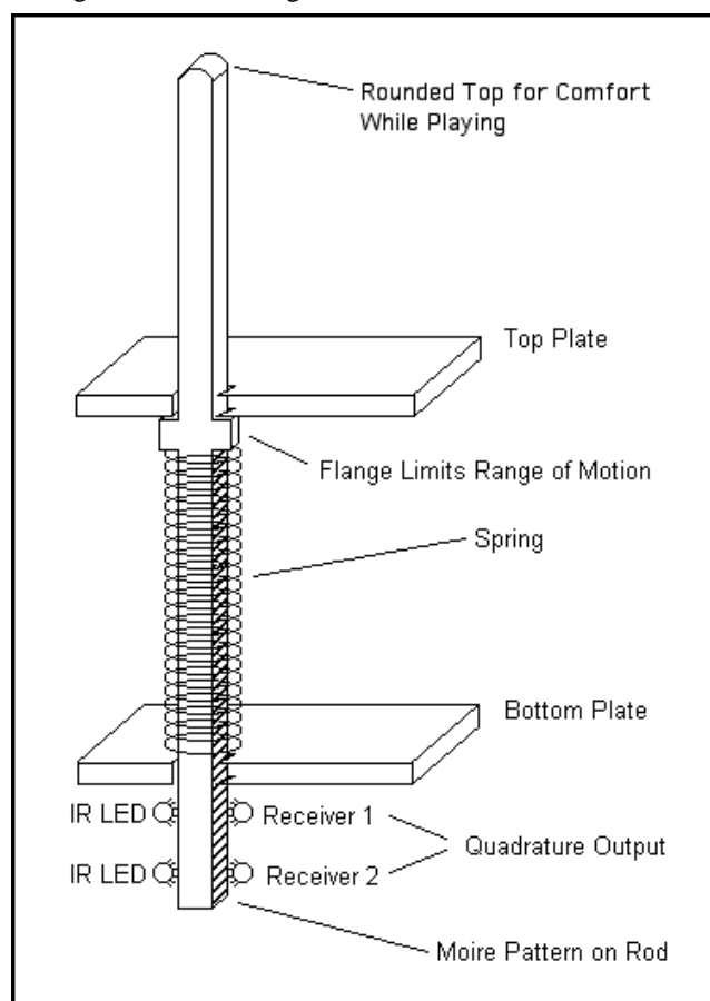
Figure 2 Diagram of a MATRIX rod.
